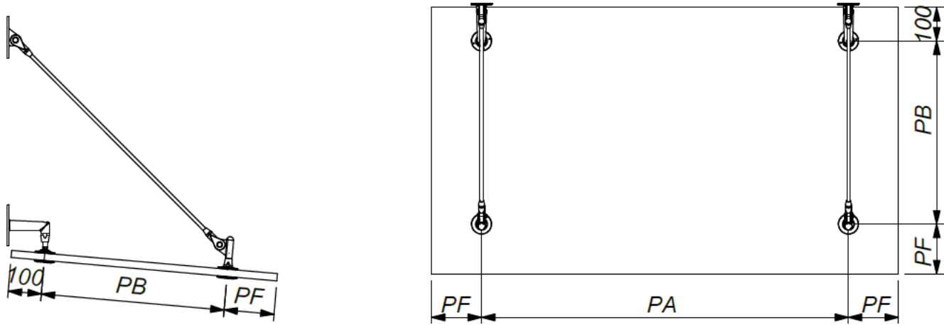
MAB&MAB Arcade baldakin
